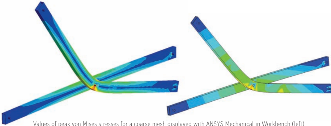
Values of peak von Mises stresses for a coarse mesh displayed with ANSYS Mechanical in Workbench (left) and with Mechanical APDL /POST1 (right). The upper support beam is shown to be bent by the applied load, simulating the effect of high winds on the sunshade.
